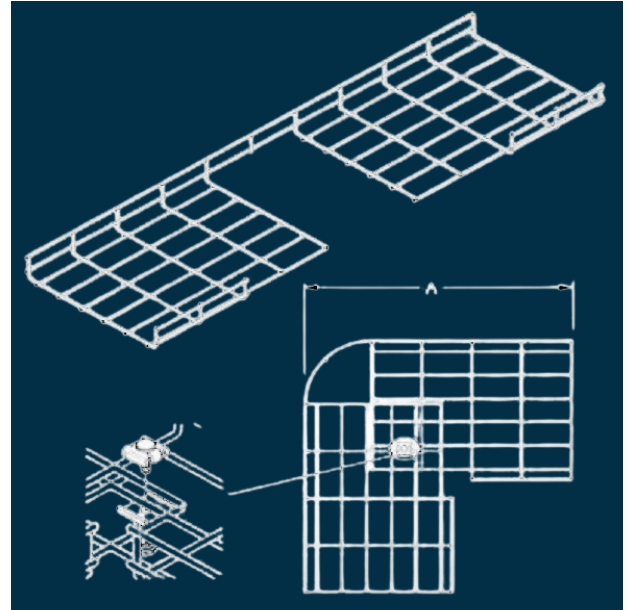
ELBOW 300
