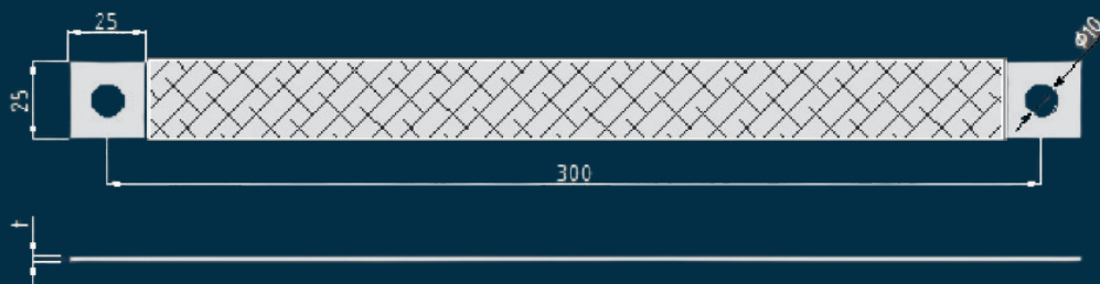
BONDING JUMPER
