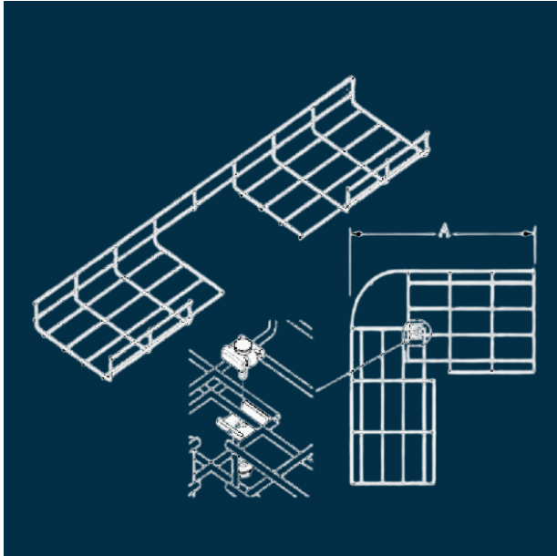
ELBOW 200
