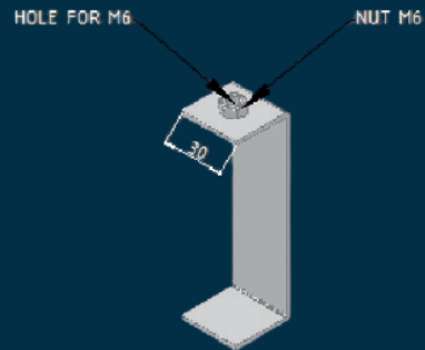
COVER CLAMP FOR HEAVY DUTY
