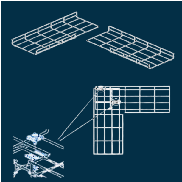
ELBOW 2 STRAIGHT
